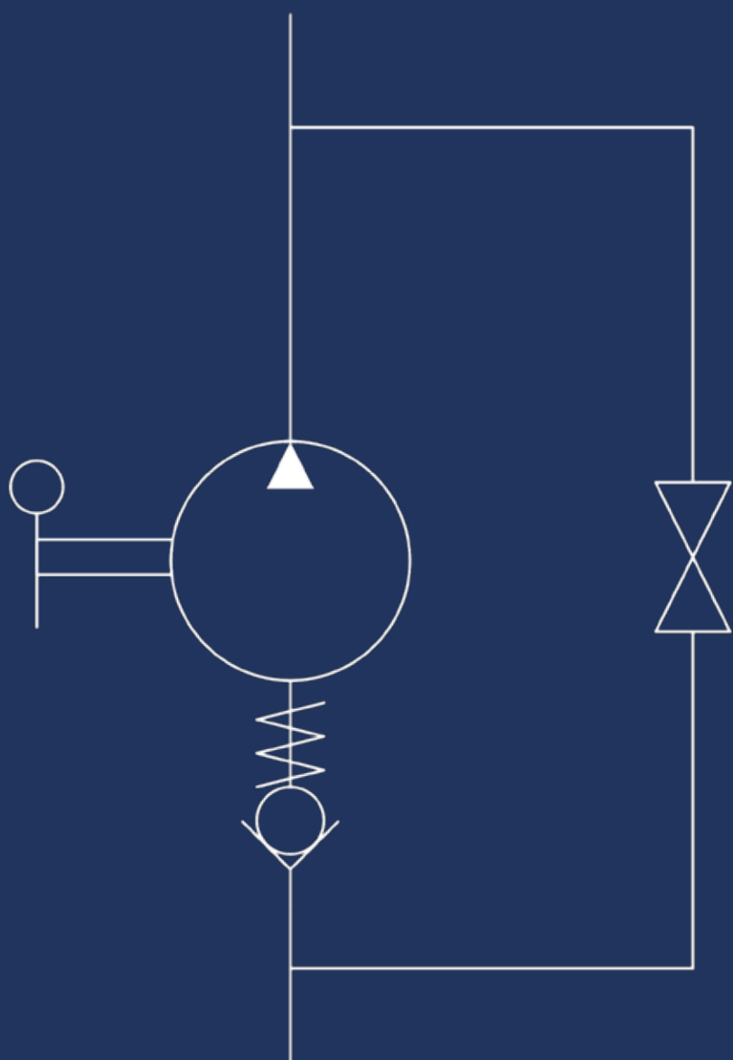
HYDRAULIC DIAGRAM
